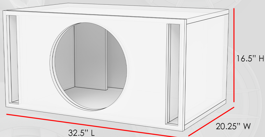
REVO 15xxx 3.0 ft 3 Ported Outer Double Baffle
